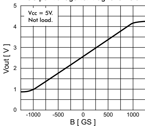
Output Voltage vs. Magnetic Field
